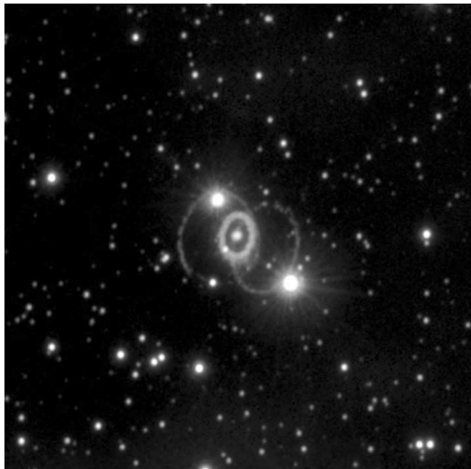
Figure 7.2 The rings around Supernova 1987A. The rings arise in gas that was expelled by the star prior to the supernova explosion. The gas in the bright “equatorial” ring was excited by the flash of UV radiation from the explosion. A delay of 240 days between the explosion and the “lighting up” of the ring was due to the light travel time from the supernova to the ring, indicating a ring radius of 240 light days. Comparison of this physical scale to the angular scale of the ring provides a direct distance measurement to the supernova, and hence to the LMC. Photo Credit: C. Burrows, ESA, and NASA.
