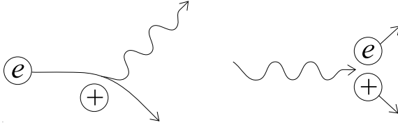
Figure 3.7 Left : A free electron accelerating in the Coulomb potential of an ion emits Bremsstrahlung, or “free-free” radiation. Right : In the inverse process of free-free absorption, a photon is absorbed by a free electron. The process is possible only if a neighboring ion, which can share some of the photon’s momentum, is present.
