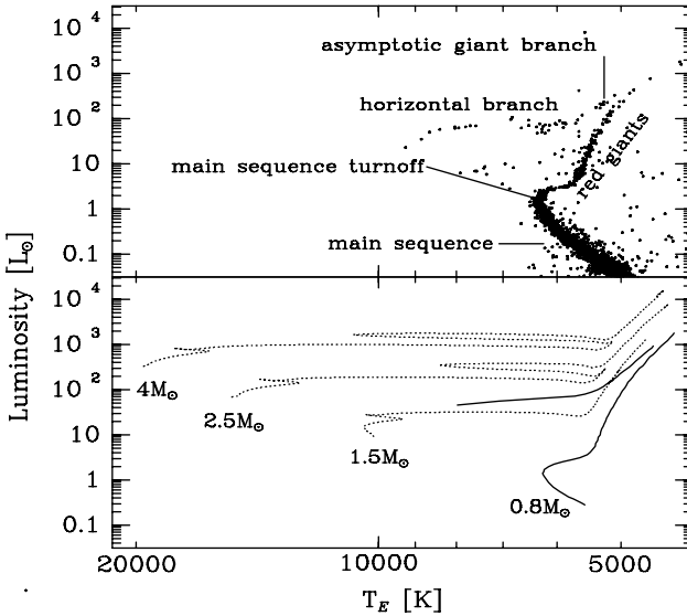
Figure 4.1 Illustration of post-main-sequence evolution on the H-R diagram. Top : Observed H-R diagram for stars in the “globular cluster” M3 (more on star clusters in Chapter 5.1.5). The main sequence turnoff marks the point at which stars are now leaving the main sequence and evolving on to the red-giant branch. All the stars in the cluster formed together about 13 Gyr ago, and the cluster has not experienced subsequent star formation. As a result, all stars above a certain mass, corresponding to the turnoff point, have left the main sequence, while those below that mass are still on the main sequence. The density of points in each region of the diagram reflects the amount of time spent by stars in each post-main-sequence evolution stage. Bottom : Theoretical stellar evolution tracks for stars of various initial main-sequence masses (with an assumed initial metal abundance of Z = 0.0004 ). Each track begins at the lower left end on the “zero-age main sequence”. After leaving the main sequence, stars evolve along, and up to the tip of, the red-giant branch. They then move quickly on the diagram to the left edge of the “horizontal branch”, where helium core burning and hydrogen shell burning take place, and evolve to the right along the horizontal branch. Once all the helium in the core has been converted to carbon and oxygen, the star rises up the “asymptotic giant branch” where double shell burning – a helium-burning shell within a hydrogen burning shell – takes place. Note the good correspondence between the theoretical track for the 0.8M_{\odot} initial-mass star (solid line) and the observed H-R diagram on top. For clarity, the theoretical horizontal and asymptotic giant branches are not shown for the other initial masses. Data credits: S.-C. Rey et al. 2001, Astrophys. J. , 122, 3219; and L. Girardi, et al. 2000, Astron. & Astrophys. Suppl. , 141, 371.
