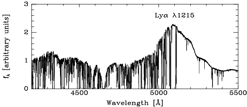
Figure 9.7 A high-resolution spectrum of a quasar at redshift z = 3.18 , with the Lyman \alpha emission line redshifted to 5080 Å. Note the “Lyman \alpha forest” of absorption lines starting from the peak of the emission line, and continuing in the blue (left) direction. These lines are due to Lyman \alpha absorption by neutral hydrogen atoms in gas clouds that are along the line of sight to the quasar, and hence at lower redshifts than the quasar. The few absorption lines to the red of the Lyman \alpha emission line peak are due to heavier elements and are associated with the system that produces the strong “damped Lyman \alpha ” absorption observed at \approx 4650 Å. Data credit: W. Sargent and L. Lu, based on observations with the HIRES spectrograph at the W. M. Keck Observatory.
