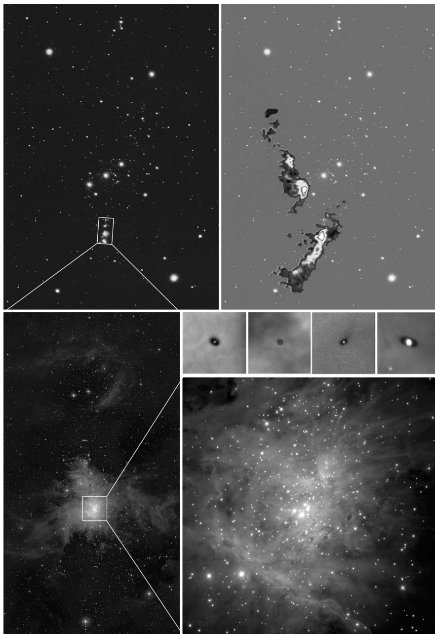
Figure 5.1 Several views of the Orion star-forming region. Counterclockwise from top pair: A map showing radio emission from the CO molecule, superimposed on an optical image of the familiar constellation; near-infrared zoom in on the region which constitutes the “sword” of the constellation, centered on the Orion nebula; a further zoom-in (about 1 pc on a side) on the “Trapezium” cluster of massive young stars that power the brightest H II region; and optical images of several protoplanetary disks around young stars, seen as dark silhouettes on the backdrop of the gas emission. Disk diameters are \sim 100 - 500 AU. Photo Credits: S. Sakamoto et al., see Astrophys. J. , 425 (1994), 641; G. Kopan, R. Hurt, and the Two Micron All Sky Survey; M. McCaughrean and the European Southern
